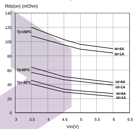
Figure 14. Static drain source on resistance
